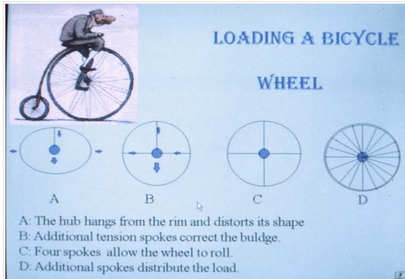
Fig. 15. The hub of a wire wheel is suspended in a tension network. The axle load is hung from the top of the rim that tries to belly out. Additional tension spokes are added horizontally to resist the bulge. For circumferential stability, the additional spokes are added. (After Fuller)
