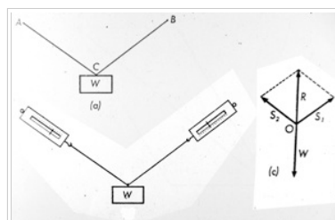
Fig. 2-2. Forces exerted by strings in supporting a weight.
