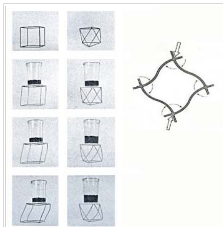
Fig. 6. The unstable square frame. Any structure that is not triangulated is inherently unstable and would require its joints to be fused to keep from collapsing. Torque and moments are created at the joints.
