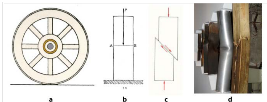
Fig. 16. Wagon wheels vault from spoke to spoke. When loaded each spoke acts as a column with compression and shear. BCD. Compression in a column creates shear stress. Therefore, the column must be thick, stiff and strong.
