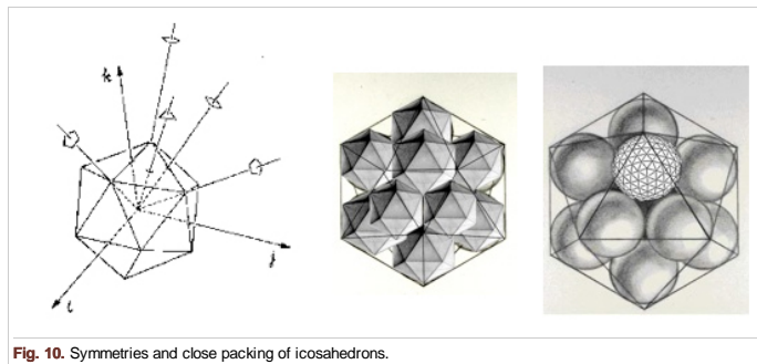
Fig. 10. Symmetries and close packing of icosahedrons.
