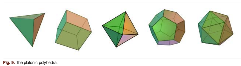
Fig. 9. The platonic polyhedra.
